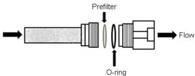
Figure 3.8 Port 1 of the LOV platform equipped with an O-ring (toric joint) and a prefilter to retain the beads.
