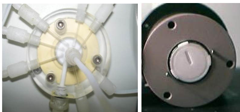
Figure 3.7 a) Left: Example of a LOV piece. b) Right: Rotor of the SV.
