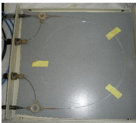
Figure 3.10 Inside of a 100 cm LWCC.
