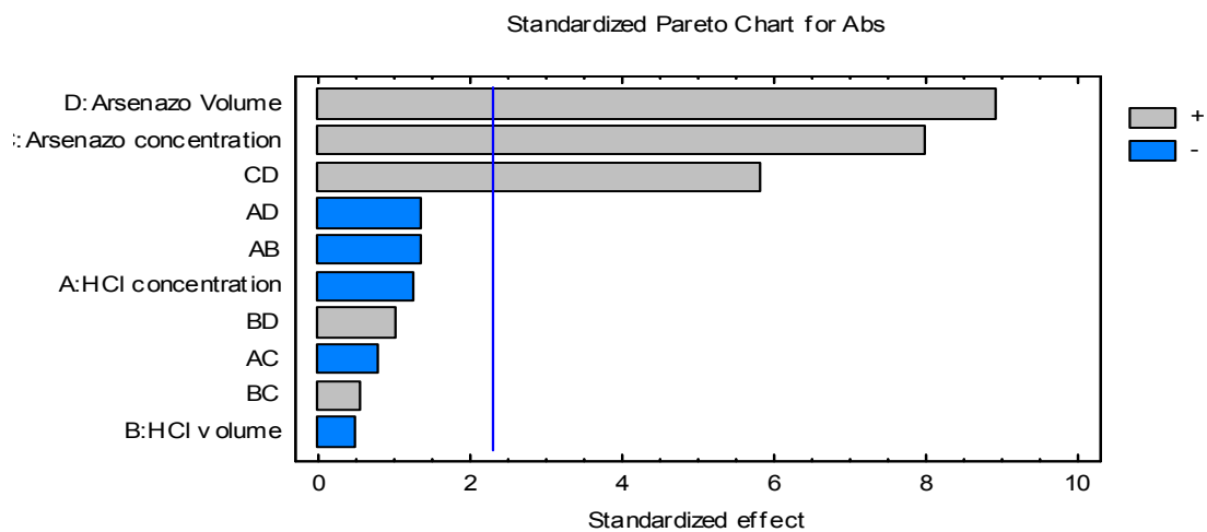
Figure 6.7 Pareto chart of the uranium screening.
