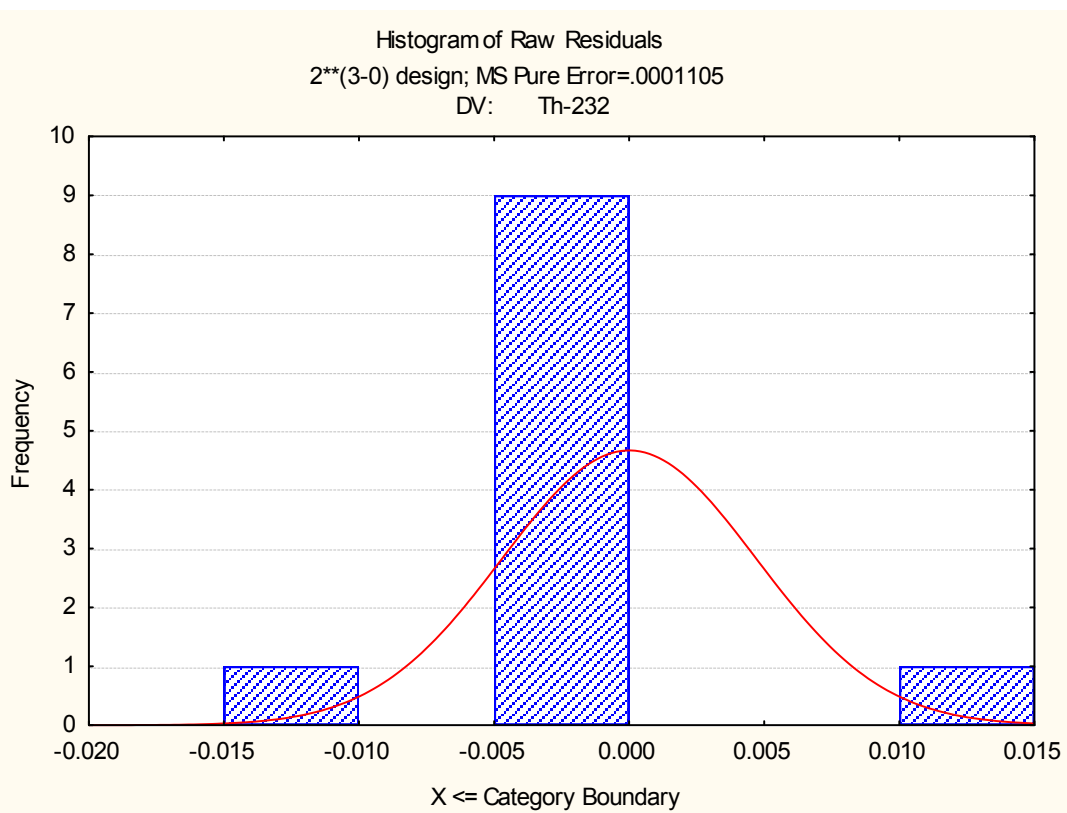
Figure 7.7 Histogram of raw residuals of the screening of ^{232}\text{Th} .
