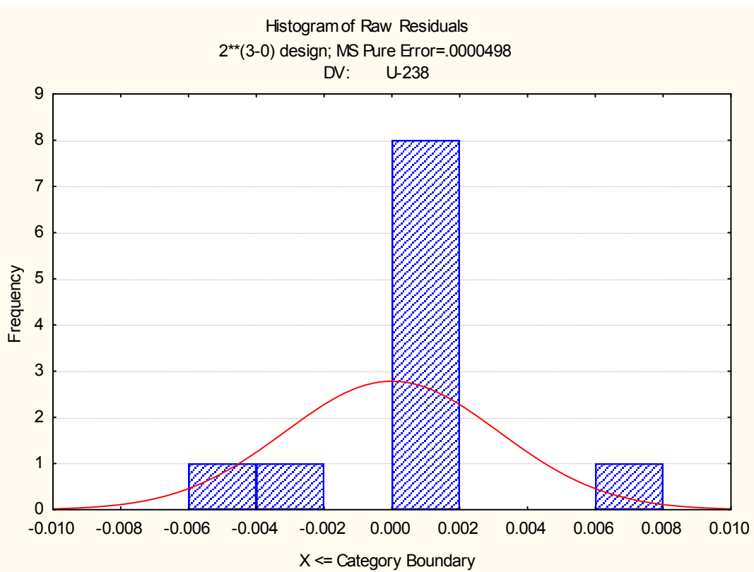
Figure 7.6 Histogram of raw residuals of the screening of ^{238}\text{U} .
