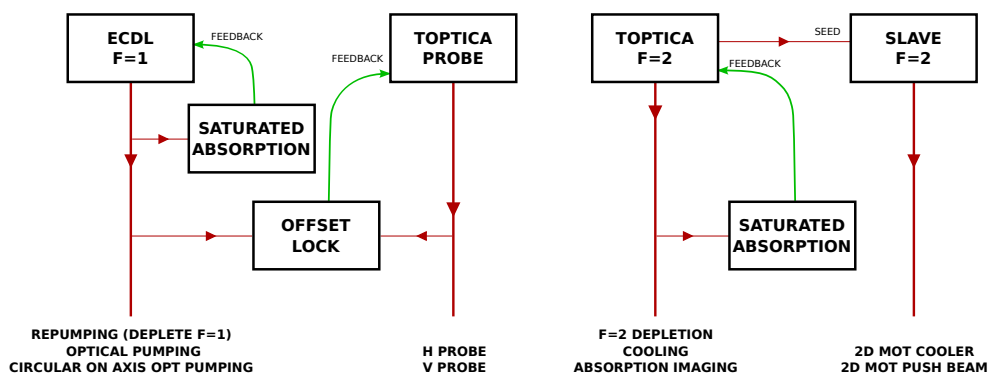
Figure 9.2: Laser system. See text for details.
