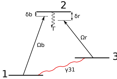
Figure 6.1: The different free parameters of the model and the levels involved. In the case of \text{Sr}^+ the levels are 1: ^5\text{S}_{1/2} , 2: ^5\text{P}_{1/2} , 3: ^4\text{D}_{3/2}
