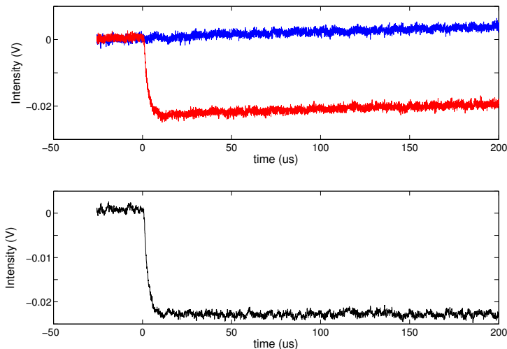
Figure 7.3: Typical absorption signal obtained at a given probe detuning (offset subtracted). Top: Photodiode signals. Blue (top): V_{p1}(t) , red (bottom) V_{p2}(t) . Bottom: difference signal used for analysis (see text for details).
