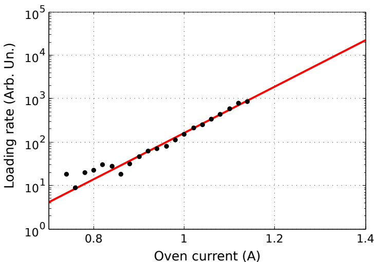
Figure 4.3: Loading rate versus oven current.
