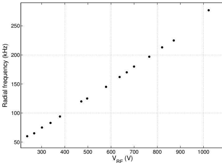
Figure 4.1: Radial frequency versus V_{RF} .
