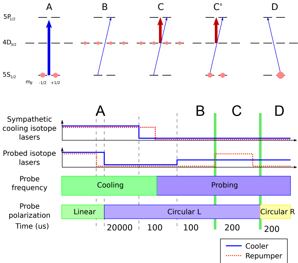
Figure 7.8: Experimental sequence used to prepare and probe the atomic system. A: The atoms are pumped to the metastable level. B: The repumper is switched off, then the probe beam frequency, polarization and power are adjusted, letting time for the photodiode transient to relax (millisecond timescale). C: The repumper is switched back on. The population is quickly (in less than 1 \mu\text{s} ) pumped into the ground level. Immediately after (C'), we observe a decrease of the probe power due to the atoms sent back to the m_F = -1/2 ground sublevel, then the probe progressively pump the atoms into the m_F = +1/2 ground sublevel. D: The polarization of the probe is switched to measure the absorption from the atoms in the m_F = +1/2 sublevel. The repumper can be switched on or off during this phase in order to isolate the specific features due to the 3-level scheme.
