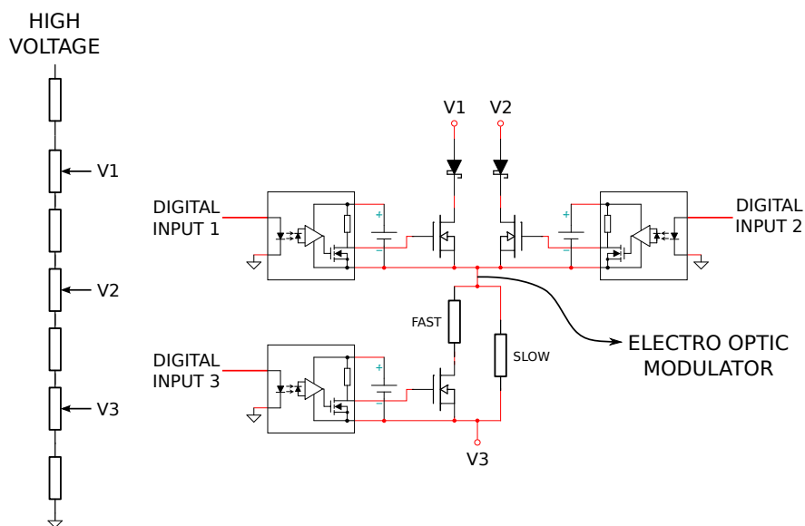
Figure 3.19: Circuit for the fast commutation of the Electro Optic Modulator. Each transistor commutes a voltage to the electrode. The bottom transistor is needed for faster switching from high to low voltages. The three voltages are made by a resistor bridge with fine tuning provided by variable resistors. The transistors (STP4N150) are driven using an external TTL signal through optoisolators (A6N37) which are powered with batteries to avoid isolation issues. The stabilization capacitors between the voltage bridge and the transistors are omitted on this sketch.
