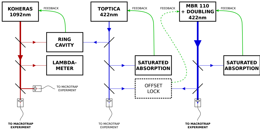
Figure 3.11: Overview of the laser system and feedback
