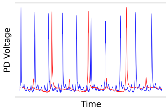
Figure 3.14: Typical traces at the output of the cavity when the lasers are locked and the cavity is spanning. In red the signal from the 1092 nm laser, in blue the signal from the 422 nm laser. The minor peaks corresponds to higher order spatial modes.
