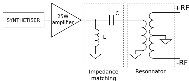
Figure 3.5: Circuit for impedance matching between the amplifier and the resonator
