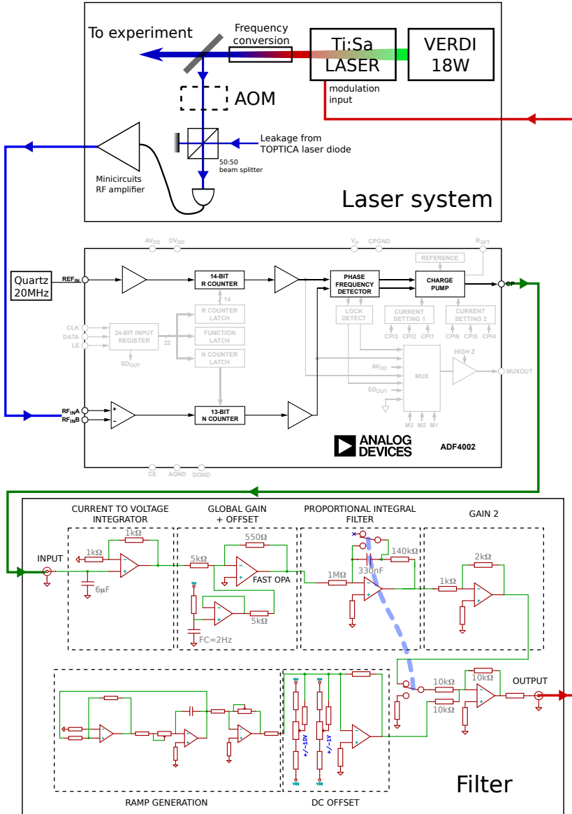
Figure C.1: Offset lock general scheme
