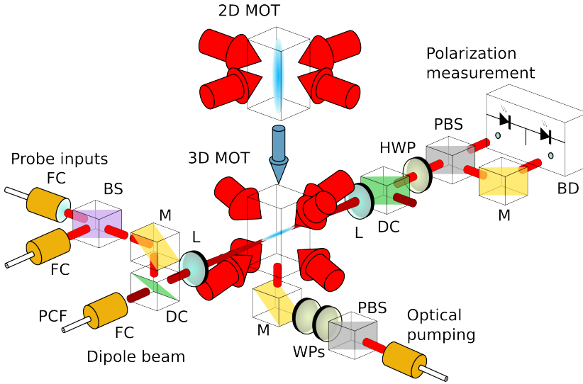
Figure 9.1: Presentation of the experimental setup. See text for details. On axis optical pumping is not represented on this figure.
