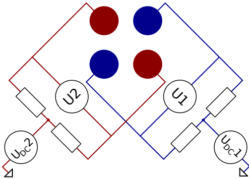
Figure 3.8: Connection of the four DC voltages to each RF electrode. The bias tee circuit is not represented on this figure.
