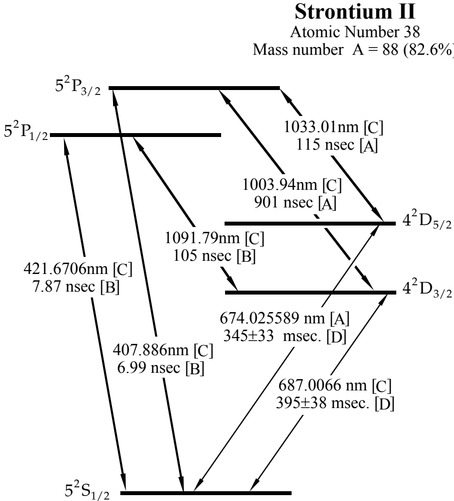
Figure D.2: Sr II transitions from [James 97]
