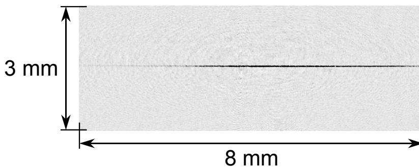
Figure 9.3: Absorption image of a typical atom cloud trapped in the dipole trap. The cloud contains about 1 \times 10^6 atoms.
