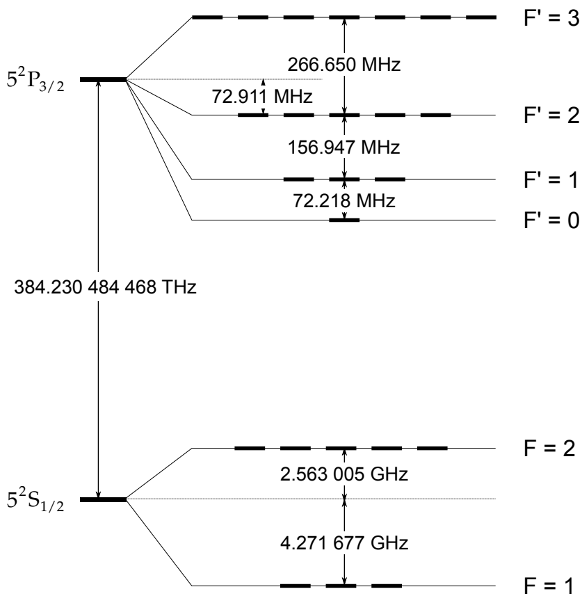
Figure B.1: ^{87}\text{Rb} D 2 line [Steck 03]
