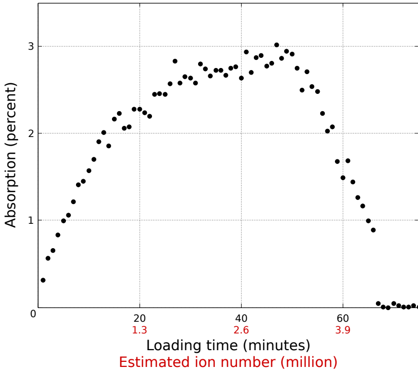
Figure 7.13: Absorption on resonance versus the ion-number in the trap (ion number estimated with the loading rate). Four phases can be identified: A first phase where the ion cloud is radially smaller than the beam cross-section and the absorption increases significantly with the number of ions. A second phase where the cloud has a size comparable to the beam cross section where the absorption increases slowly due to the increasing ion cloud length (and a possible slight misalignment of the probe). A third phase, where the absorption drops significantly, which can be understood as an increase of cloud temperature from radio-frequency heating that affects the peripheral ions. Then more drastic absorption drop is noticed, the observation of the cloud images show a simultaneous loss of the "dense" phase. This phenomenon can be interpreted by an insufficient cooling to keep the dense phase cold enough.
