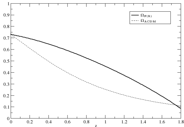
Figure 6.2: Evolution of the cosmological parameter from dark energy versus redshift, such for F(R) theory as for \Lambda\text{CDM} model.
