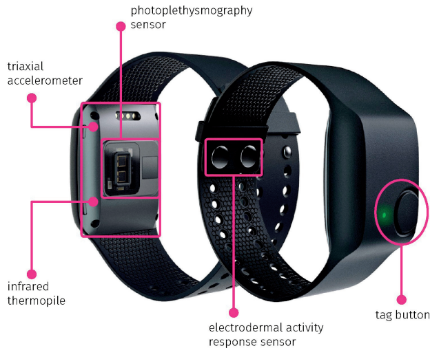
Figure 7. E4 wristband, overview of sensors (adapted from Empatica.com)
