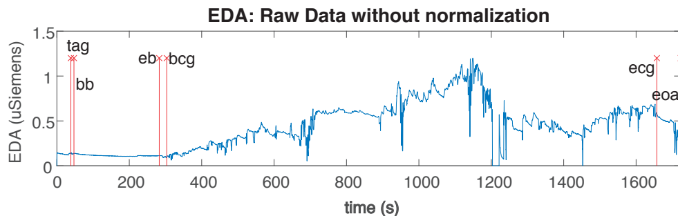
Figure 11. Example of invalid EDA signal. The vertical red lines indicate the different phases of the activity: tag, bb: beginning baseline, eb: end baseline, bcg: beginning cognitive games, ecg: end cognitive games, eoa: end of activity
