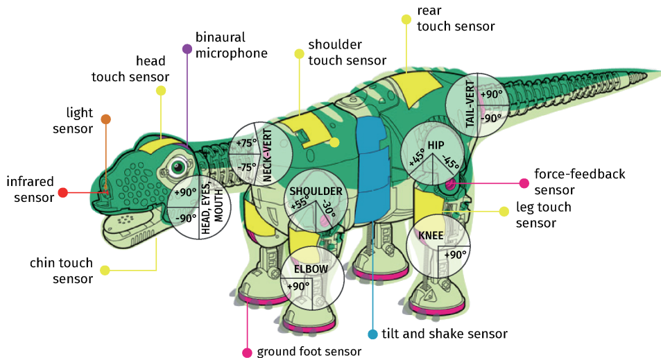
Figure 6. Pleo, overview of sensors and degrees of freedom (adapted from L-DOPA)
