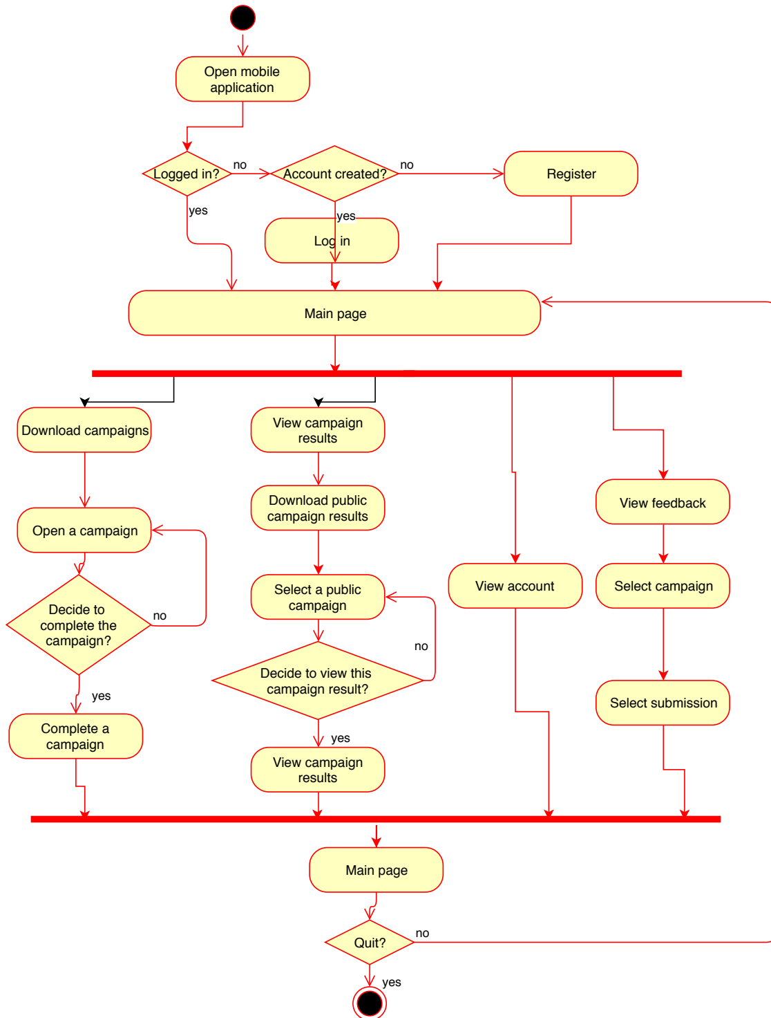
Figure 3.8: Activities performed by the data collectors using the mobile application.
