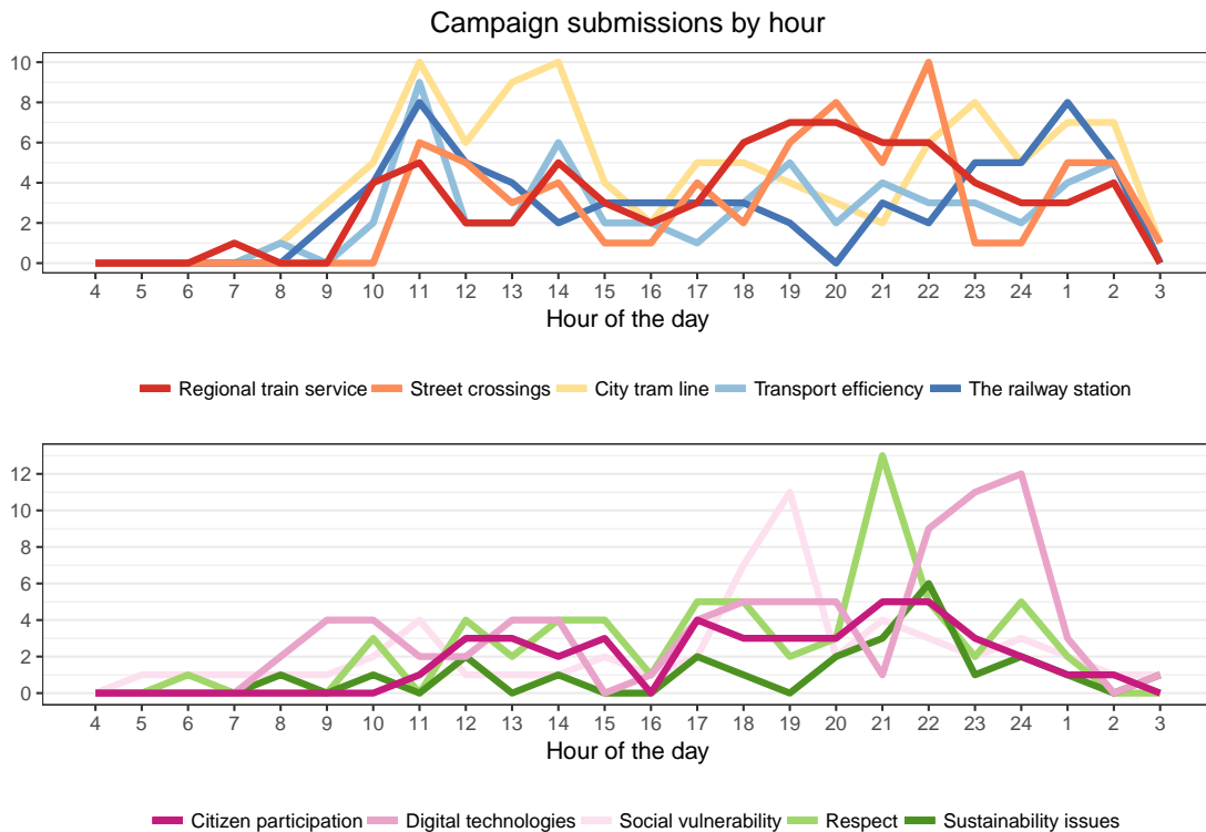
Figure 6.4: The distribution of submissions from different campaigns throughout the deployment rendered in a 24-hour time frame. (upper) The campaigns having different patterns than the overall submission pattern. (lower) The campaigns having a similar pattern to the overall submission pattern.
