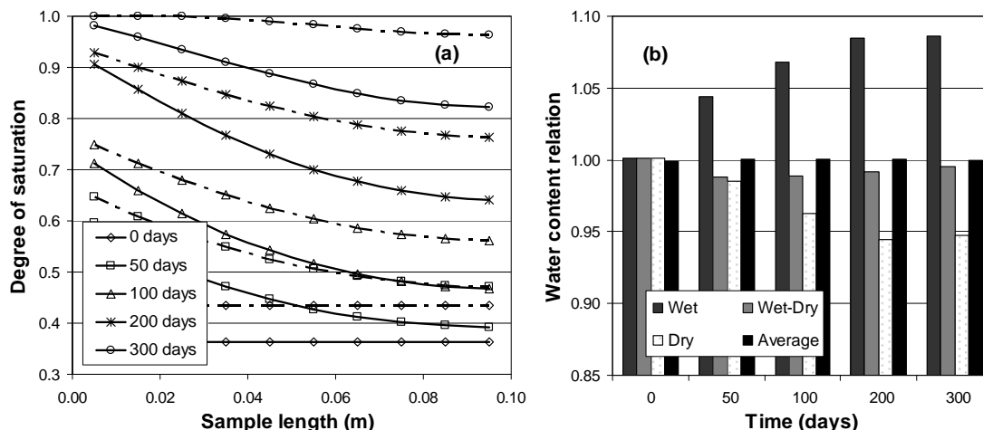
Figure 4.10. (a) Evolution of the degree of saturation at different times and for each case considered; continuous lines correspond to Case 1 and dotted lines to Case 2; (b) temporal evolution of the relation between values of water content at different zones within the sample.
