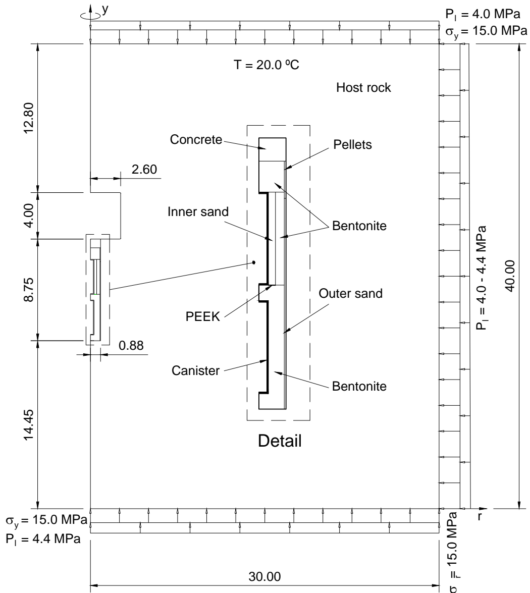
Figure 6.8. Axisymmetric geometry for the analysis of the in situ heating test (dimensions are in meters).
