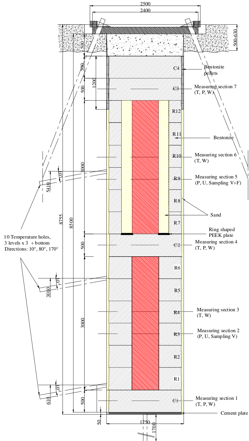
Figure 6.3. Experimental set up of the Temperature Buffer Test (SKB, 2005).
