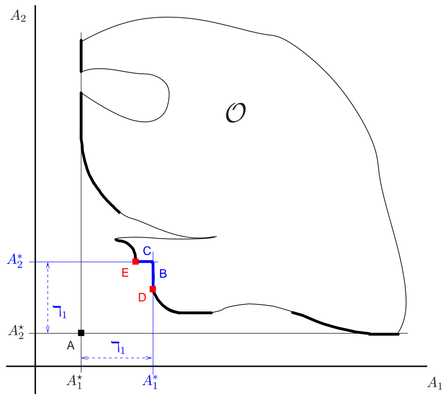
Figure VI-16: Example of a multiple solution case using the lexicographic egalitarian optimisation strategy for a two criteria multi-objective minimisation problem
