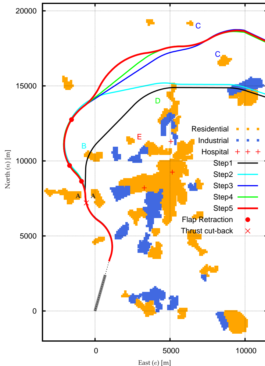
Figure VI-9: Significant intermediate steps in the optimisation process for the Airbus A340 during night periods (04h)
