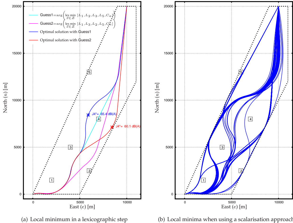
Figure V-11: Examples of local minima
