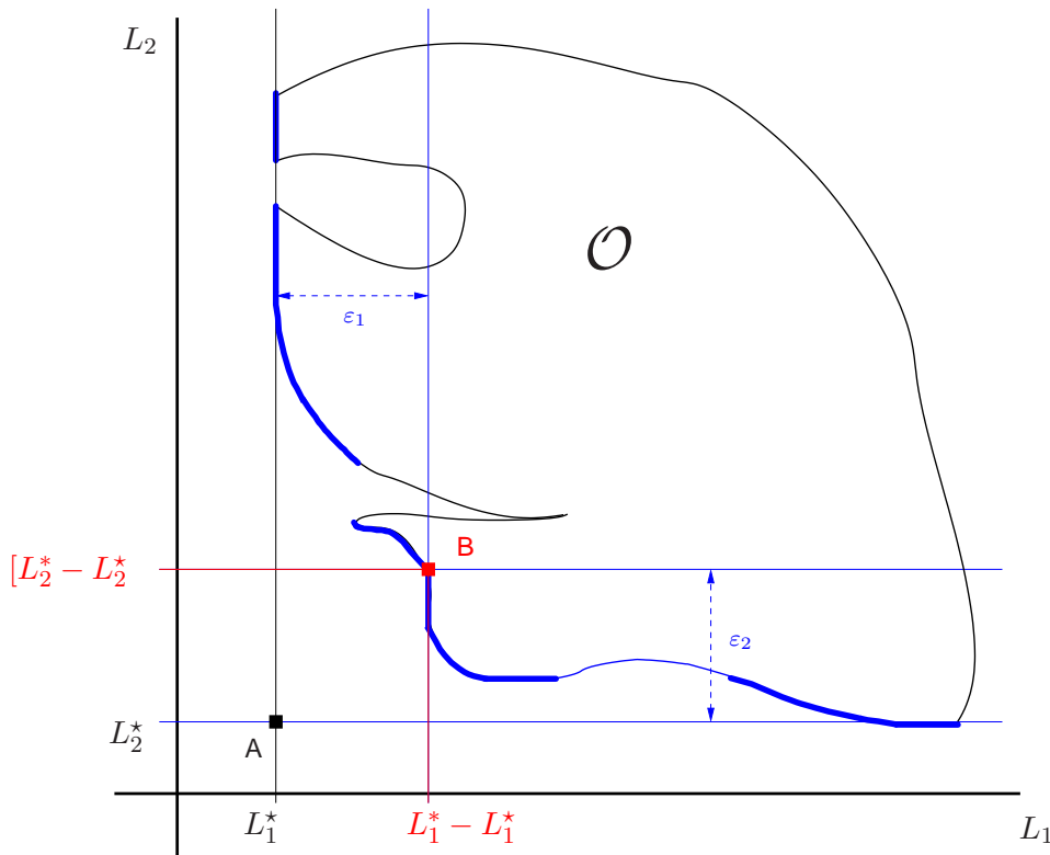
Figure V-12: Example of Tchebycheff optimisation strategy for a two criteria multi-objective minimisation problem
