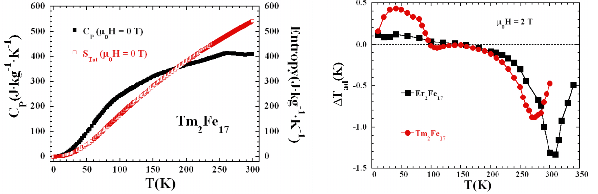
Figure 3.10: Left plot: Temperature dependence of the total entropy and heat capacity of the Tm_2Fe_{17} at \mu_0 H = 0 T. Right plot: Temperature dependence of the \Delta T_{ad} at a maximum applied field of 2 T for the Er_2Fe_{17} and Tm_2Fe_{17} compounds.
