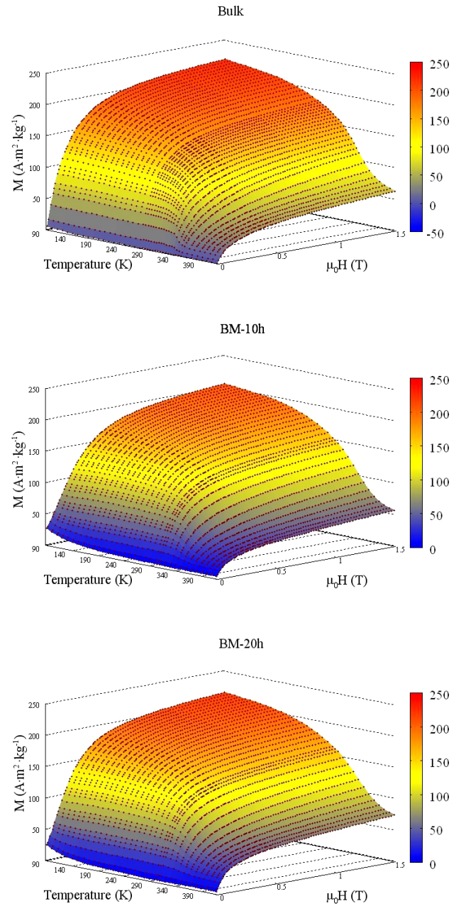
Figure 3. Temperature and applied magnetic field dependencies of the magnetization for the bulk and milled \text{Nd}_2\text{Fe}_{17} samples.
