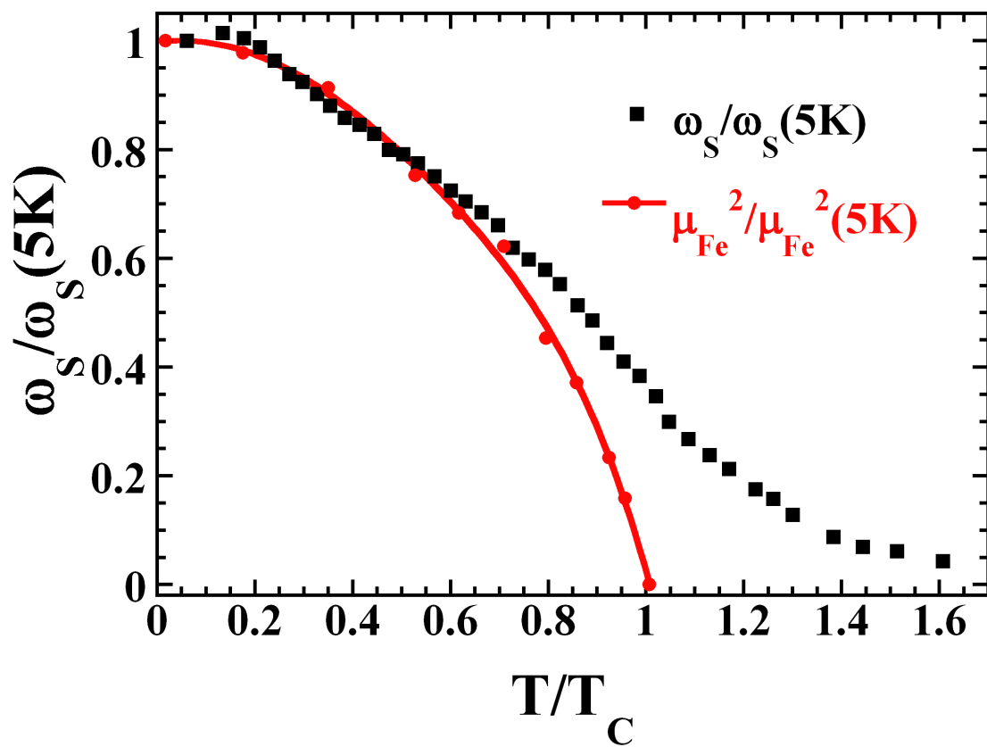
Fig. 5 Reduced volume effect \omega_s(T) / \omega_s(5\text{ K}) on the reduced temperature T/T_C compared with the temperature dependence of the square of the magnetic moment of \text{Er}_2\text{Fe}_{17} .
