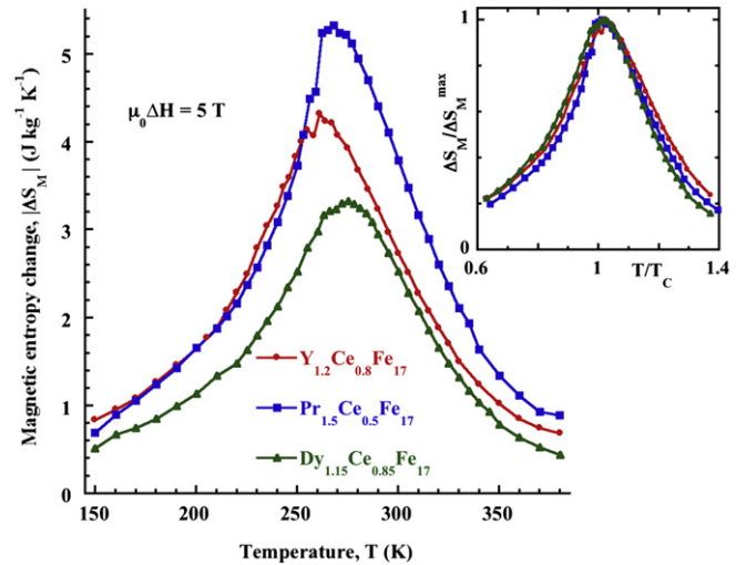
Fig. 5. Temperature dependence of the magnetic entropy change for the maximum applied magnetic field change \mu_0 \Delta H = 5 T. The inset shows the normalized |\Delta S_M| vs T/T_C curves.
