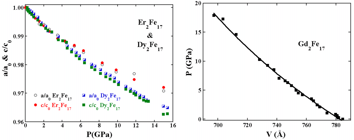
Figure 3.7: Left plot: Pressure dependence of the normalized cell parameters for the rhombohedral Dy_2Fe_{17} and hexagonal Er_2Fe_{17} alloys. Right plot: Pressure as a function of cell volume of Gd_2Fe_{17} alloy, fitted with eq. 3.2.
