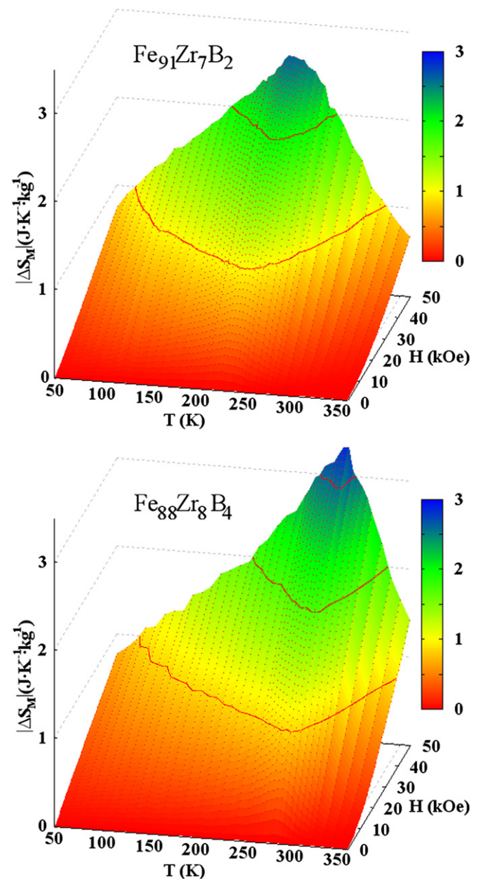
Fig. 2. Temperature and magnetic field dependences of |\Delta S_M| for B2 and B4 samples.
