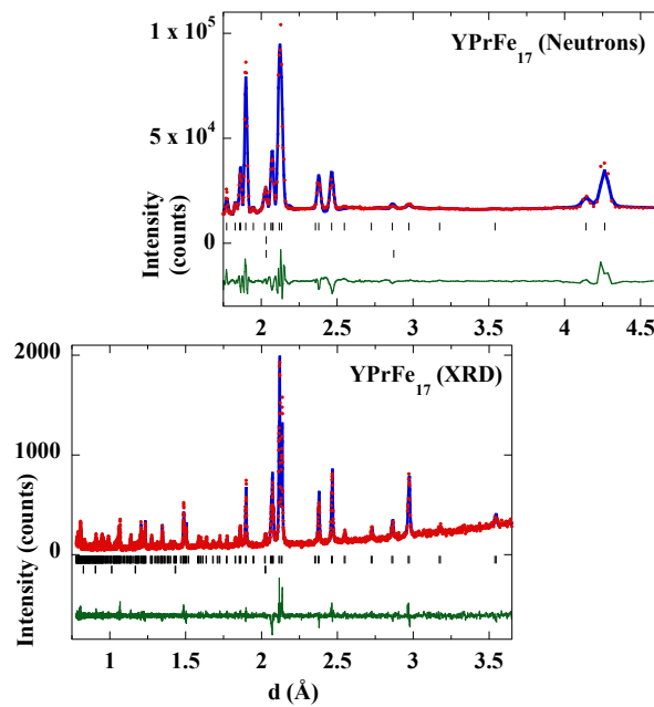
Fig. 1. Observed (dots) and calculated (solid line) powder diffraction patterns for YPrFe_{17} alloy collected at T = 300 K. Positions of the Bragg reflections are represented by vertical bars; the first row corresponds to the rhombohedral Th_2Zn_{17} -type phase while the second one is associated with an \alpha -Fe impurity ( < 3\% ). The observed–calculated difference is depicted at the bottom of each figure.
