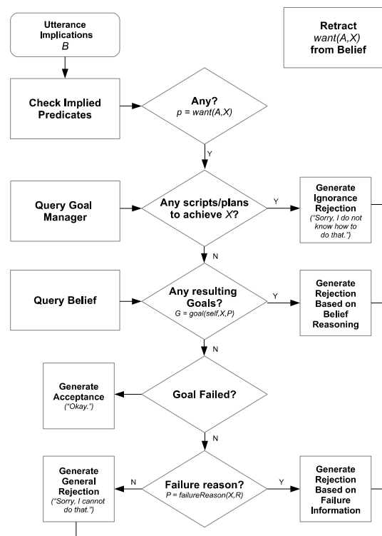
Generate Acceptance/Rejection Process
