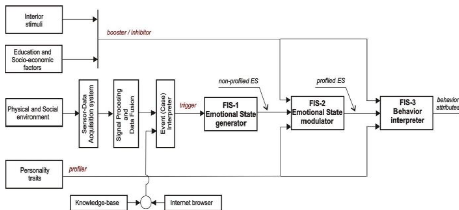
Figure 53 Emotion Based Model in Mihaljo Pupin Robot.
