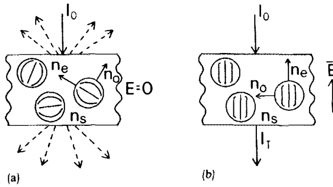
Fig 2.3.3-2 Schematic of random (a) and ordered (b) alignment under off and on state of external E field [21]
