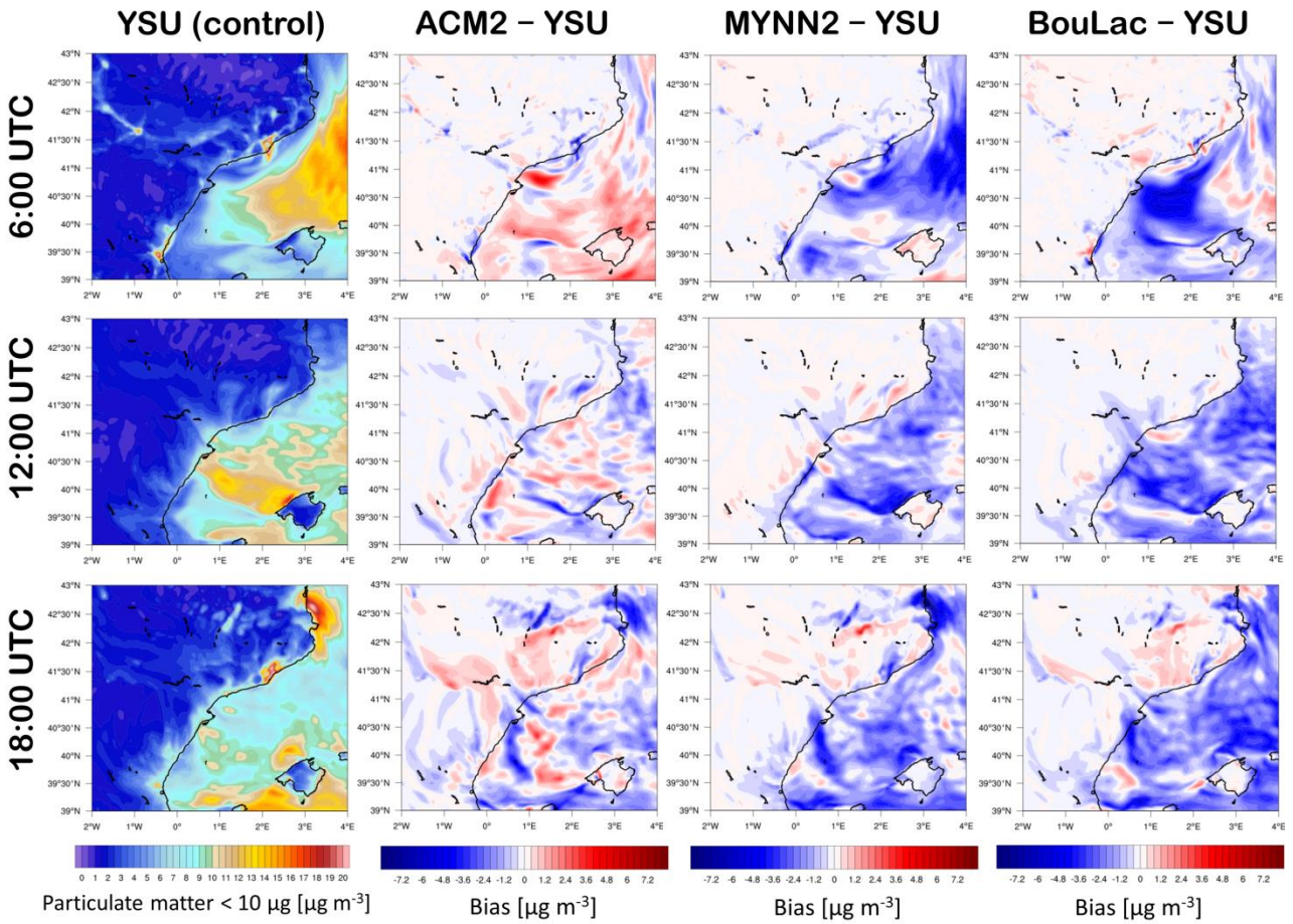
Figure 5.8 Same as in Fig. 5.6, except for surface concentration of particulate matter < 10 \mu\text{m} ( PM_{10} ).
