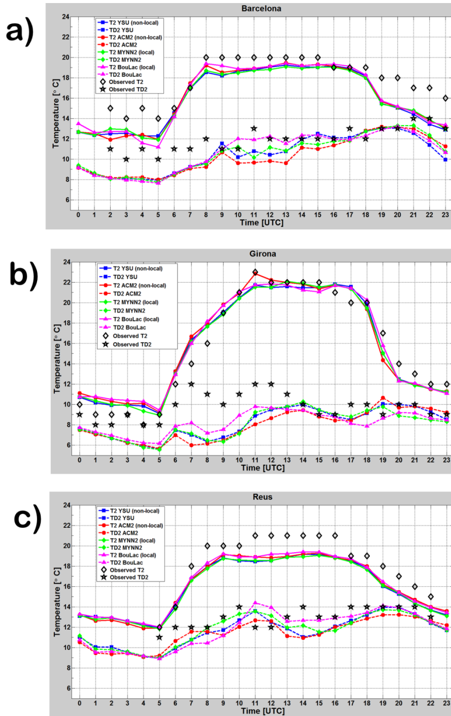
Figure 5.3 Time series on 7 May 2015 of WRF model-simulated 2-m air temperature (T2; solid lines) and dew point temperature (TD2; dashed lines) against METAR observations at; a) Barcelona, b) Girona, and c) Reus.
