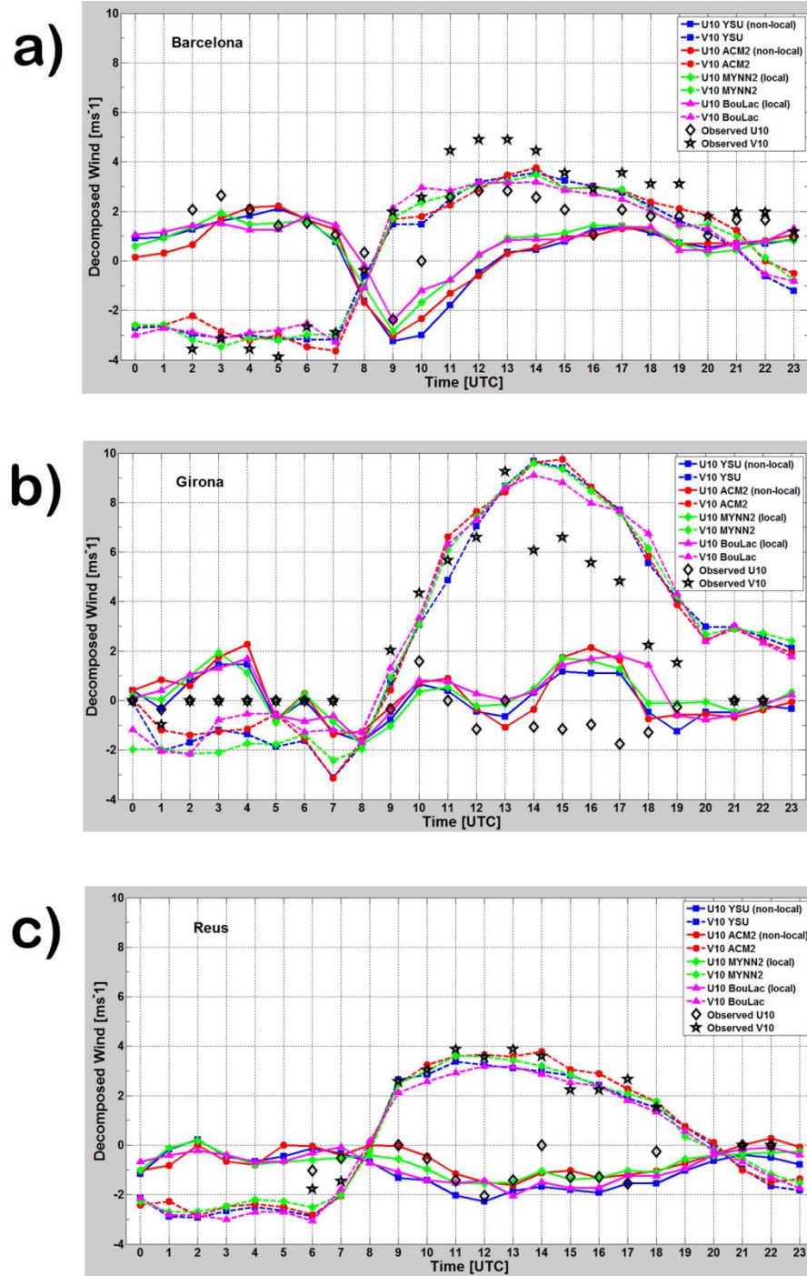
Figure 5.4 Same as in Fig. 5.3, except for zonal (U10; solid lines) and meridional (V10; dashed lines) components of 10-m winds.
