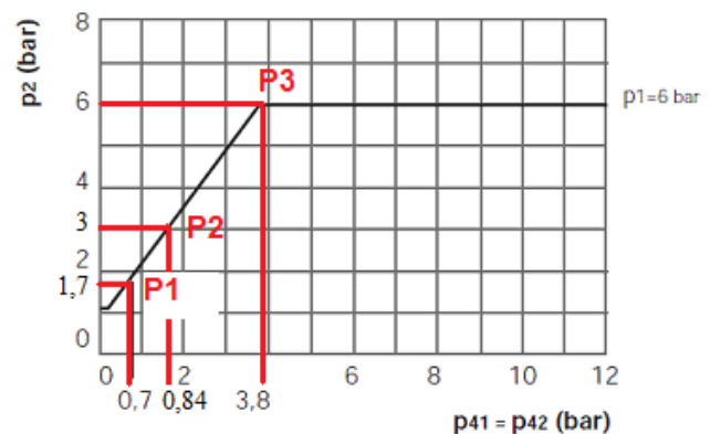
Fig. 19. LSV check points with the third point in the proportionality area.
