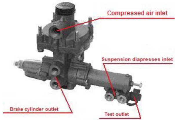
Fig. 3. Pneumatic LSV [6].
