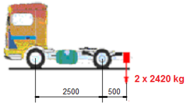
Figure 11. Test 5. IVECO tractor unit.
