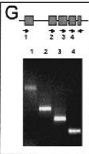
Figure 2 A new gene in Caenorhabditis elegans and Drosophila melanogaster coding for B domain-like sequences. (A) Alignment of the human UEV1 B domain with TBLASTN-identified segments from C. elegans Y53C10 and D. melanogaster DS00863 genomic clones. The aligned segments are discontinuous in Y53C10, as indicated by the positions of nucleotides from the database entry. (B) Dot-plot analysis of reciprocal TBLASTX comparisons of genomic clones Y53C10-B ( C. elegans ) and DS00863-B ( D. melanogaster ). (Bottom) Scores of sequence identities for each diagonal of conserved segments, shown as horizontal bars. (C) Predicted structure of the new gene in C. elegans (middle) supported by gene prediction algorithms (top) and alignment with ESTs (bottom). (D) Predicted C. elegans protein containing a B domain-like segment (shaded). (E) Predicted structure of the new gene in D. melanogaster (middle), supported by gene prediction algorithms (top) and alignment with ESTs (bottom). (F) Predicted D. melanogaster protein containing a B domain-like segment (shaded). (G) Expression analysis by RT-PCR, with forward primers corresponding to exons 1, 2, 3, and 4 of the predicted gene, and a reverse primer corresponding to exon 5, using as templates embryo mRNAs. (H) Cytogenetic assignment of D. melanogaster UEV gene to chromosome 3 segment 64D. Digoxigenin-labeled cDNA probes were used for hybridization on wild-type Drosophila polytene chromosomes.
