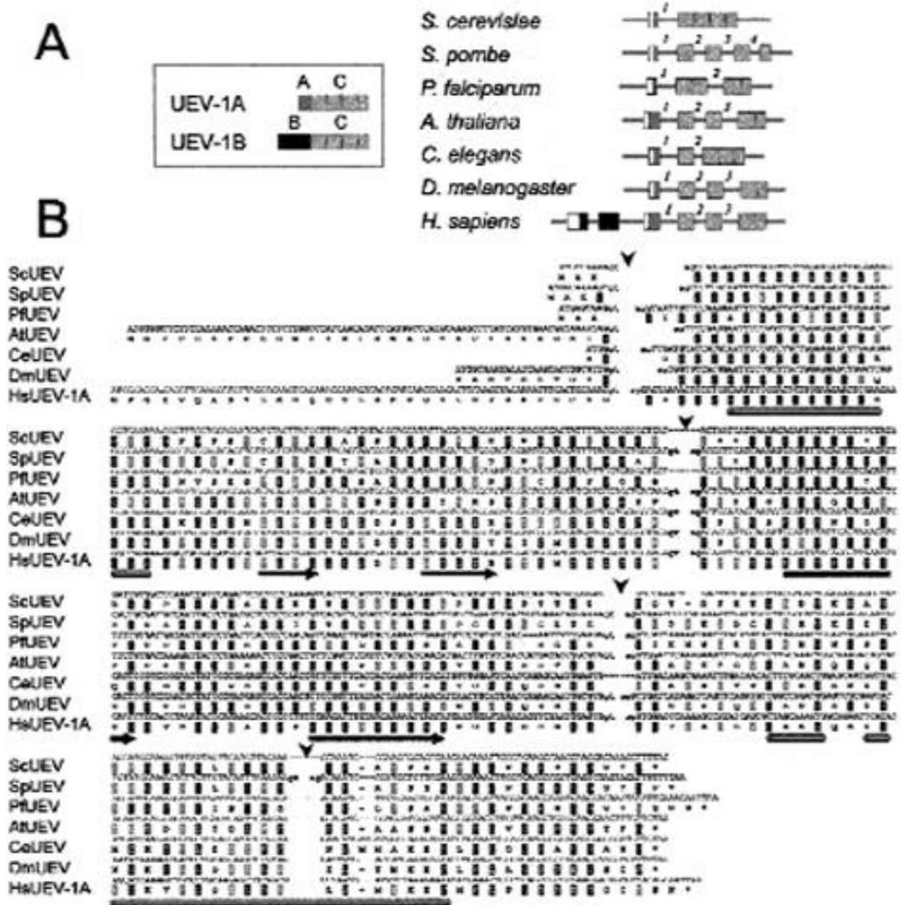
Figure 1 Conservation of introns in UEV genes from distant organisms. (A) Diagrammatic representation (not to scale) of the relative exon-intron arrangement of the UEV gene in Saccharomyces cerevisiae , Schizosaccharomyces pombe , P. falciparum , Arabidopsis thaliana , Caenorhabditis elegans , Drosophila melanogaster , and Homo sapiens . Inset diagram for the two major isoforms described for human UEV1 . Putative 5' untranslated (UTR) segments are represented as open boxes. Introns are designated by numbers that are specific for each UEV gene. Vertical dotted lines within exons define segments corresponding to the exons in S. pombe UEV . (B) Alignment of UEV genes and proteins showing precise conservation of the position of the second and third introns interrupting the C domain of UEV proteins. Splice donor and acceptor sequences in intron boundaries are in lower case. The positions of introns are marked by arrowheads. Predictions of secondary structure are shown below the sequences as rods (helices) or arrows (strands).
