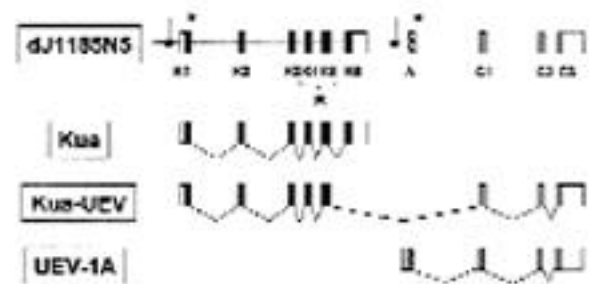
Figure 7 Diagrammatic representation summarizing the three major classes of transcriptional units generated at the Kua-UEV locus. Transcription from the promoter located upstream from the first exon of Kua can eventually yield either a Kua -only transcript ending in K6 ( Kua ), or a Kua-UEV hybrid transcript. The maturation of the longer transcript is possible only after removal of the K6 exon, which contains signals for truncation of the primary transcript. Transcription from the promoter located upstream from the A exon yields UEV1A . (Black boxes) Kua exons; (light grey boxes) UEV "common domain" exons; (shaded box) UEV "A" exon; (open boxes) 5' and 3' UTRs; (filled circles and arrows) putative transcription initiation sites.
