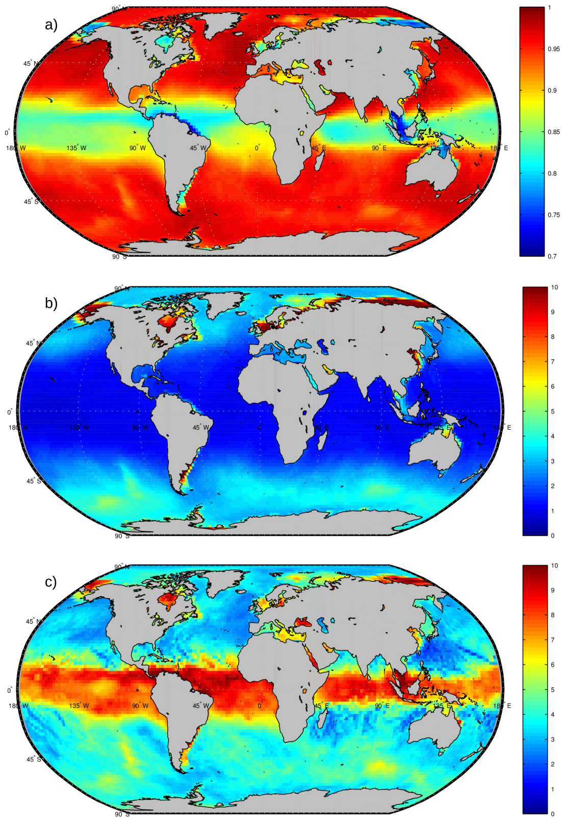
Figure 4.1: Spatial validation of the statistical reconstruction. a) correlation coefficient( \rho ). b) RMSE (cm). c) RMSE relative to the maximum surge variability(%).
