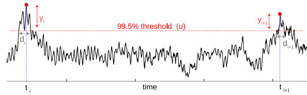
Figure 3.2: Peak over threshold technique. Red dots are extreme events, values over the 99.5%. Each of the selected extremes occurs at a specific time t_i , has a specific duration of d_i and exceeds the threshold by an amount of y_i
