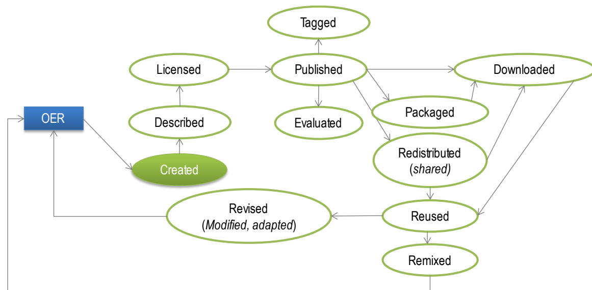
Figure 2-5. OER's lifecycle
