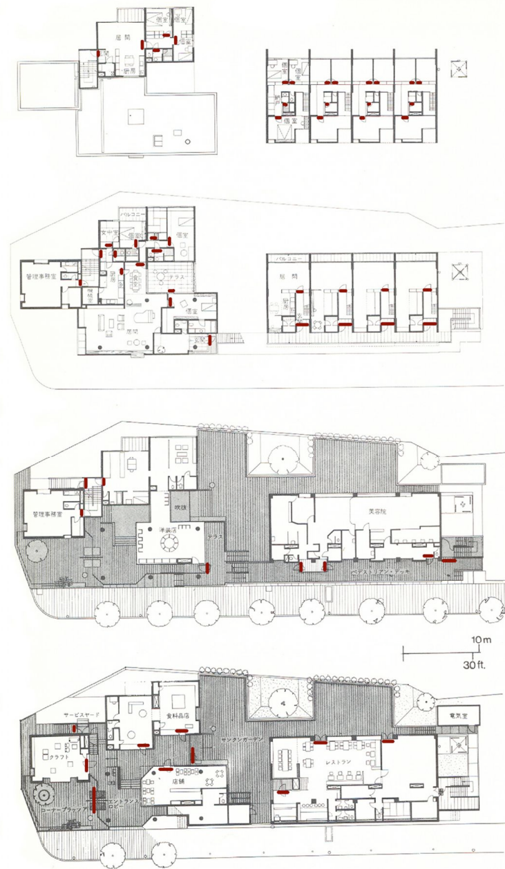
Original floorplans all levels
