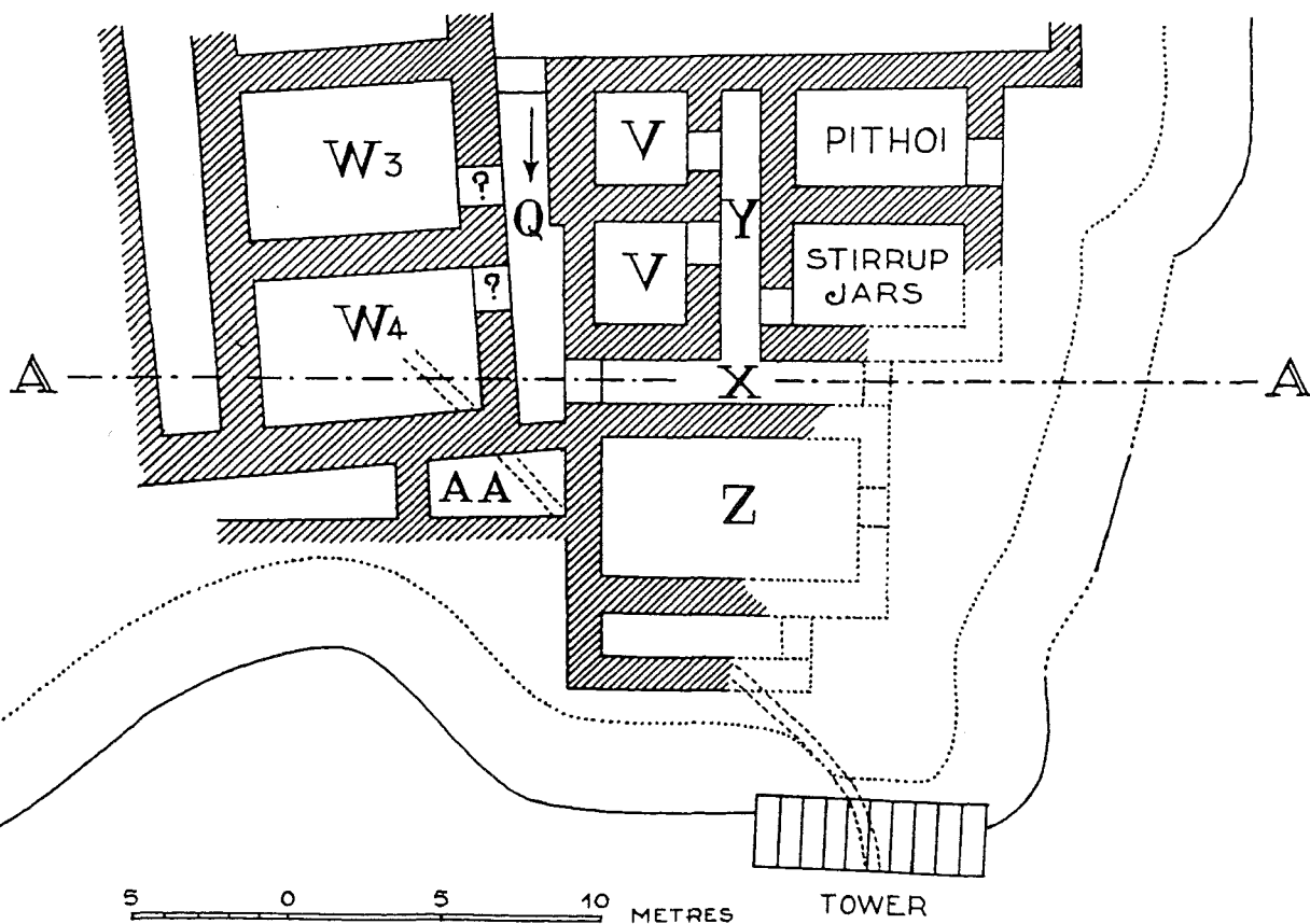
34. HOUSE OF COLUMNS, BASEMENT, plan and section
