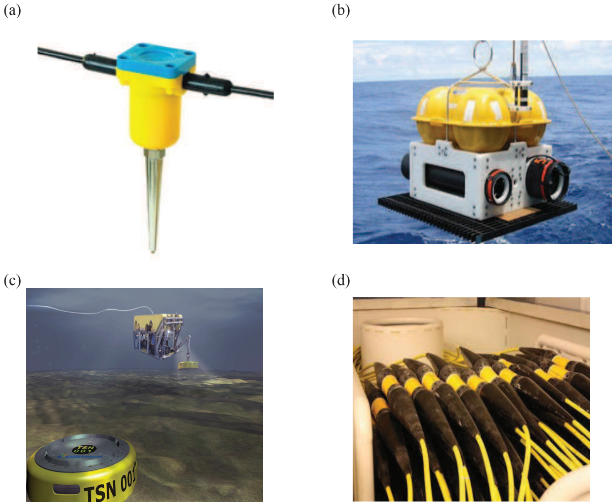
Figure 1.3. Examples of the main types of seismic receivers. (a) Geophone. For recording, the nail-like end is driven into the ground. Image from www.mitchamindustries.com . (b) OBS/H. For deployment, the device is dropped into the water and it falls to the seafloor. For recovery, it releases a weight (the metal piece attached at the bottom in the image) and it comes back up to the sea surface. Image from www.ventureddeepocean.org . (c) OBN. These compact receivers are deployed and recovered using ROVs (Remotely Operated Vehicle), and are typically laid out forming a grid. Image from www.cggveritas.com . (d) OBC. In 3-D experiments cables are usually arranged parallel to each other over the target study area. Image from www.sercel.com .
