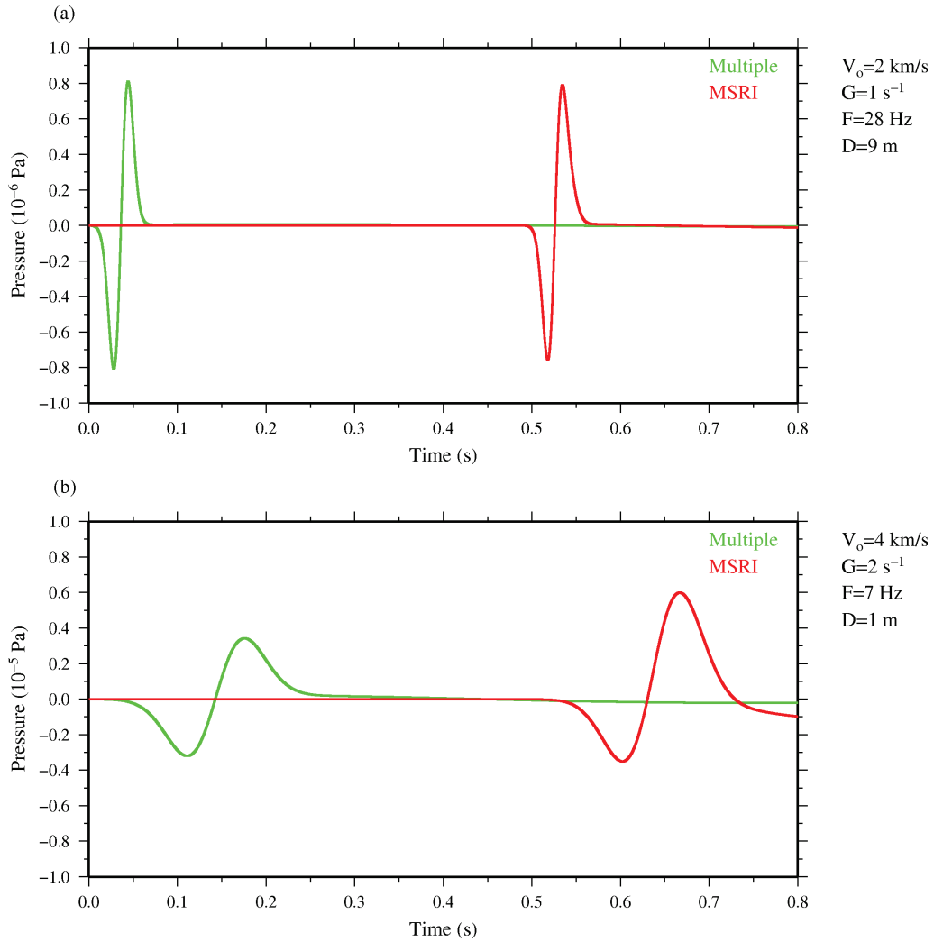
Figure 3.3. Selected examples of 1-D acoustic wave propagations performed with shot1D for (a) r_o \approx 0.98 with V_o=2 km/s, G=1 s ^{-1} , F=28 Hz, D=9 m, and (b) r_o \approx 1.75 with V_o=4 km/s, G=2 s ^{-1} , F=7 Hz, D=1 m (black circles in Fig. 3.4a and 3.4f, respectively). Green lines represent the traces recorded 1 m below the source from which we obtain the peak amplitudes of the incident multiple waves, whereas red lines represent the traces recorded at a distance D above the sea-floor which provide the MSRI peak amplitudes.
